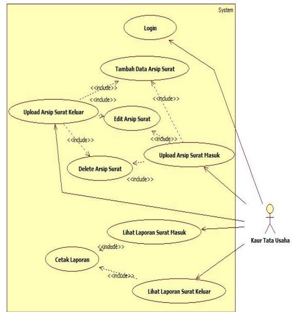
Gambar 3 : Use Case Diagram Kaur TU
